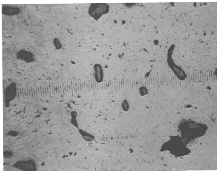
Fig. 17.--Polished GdSb Plus Unknown Substances, Type I, 200X
